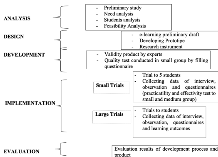
Fig. 1. Research methodology
