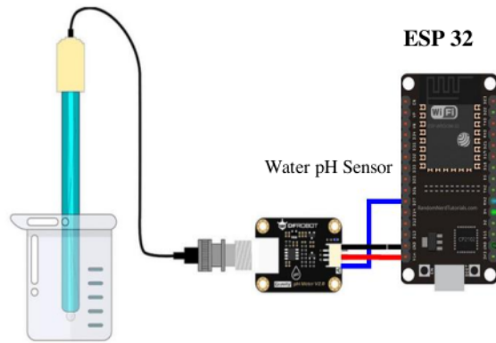
Figure 10 PH-4502C water pH sensor circuit
