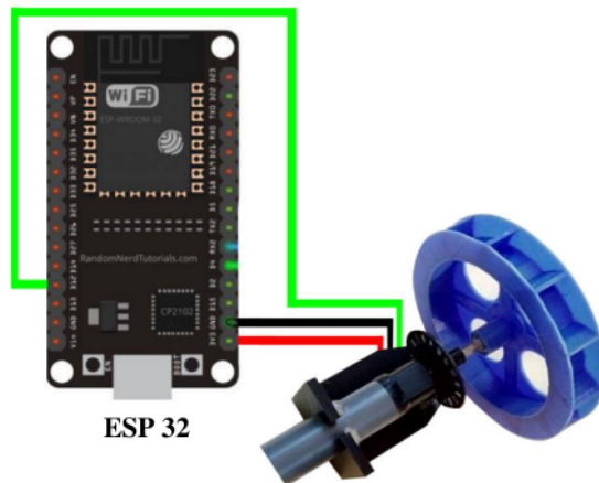
Figure 14 Water flow Sensor Circuit
