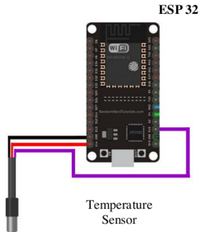
Figure 12 DS18B20 Temperature Sensor Circuit
