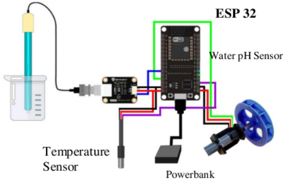
Figure 8 Hardware Sets
