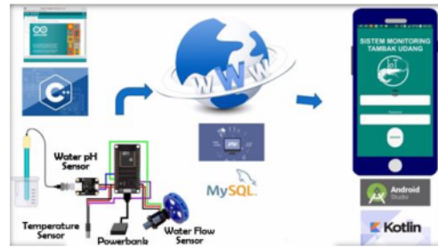
Figure 1 System design
