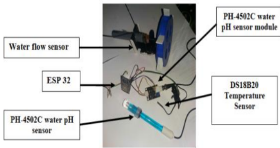
Figure 9 Hardware Device
