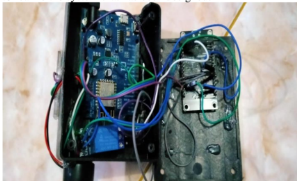
Fig. 1 Home Security Alarm Using Wemos D1 and Sensor HC-SR501
