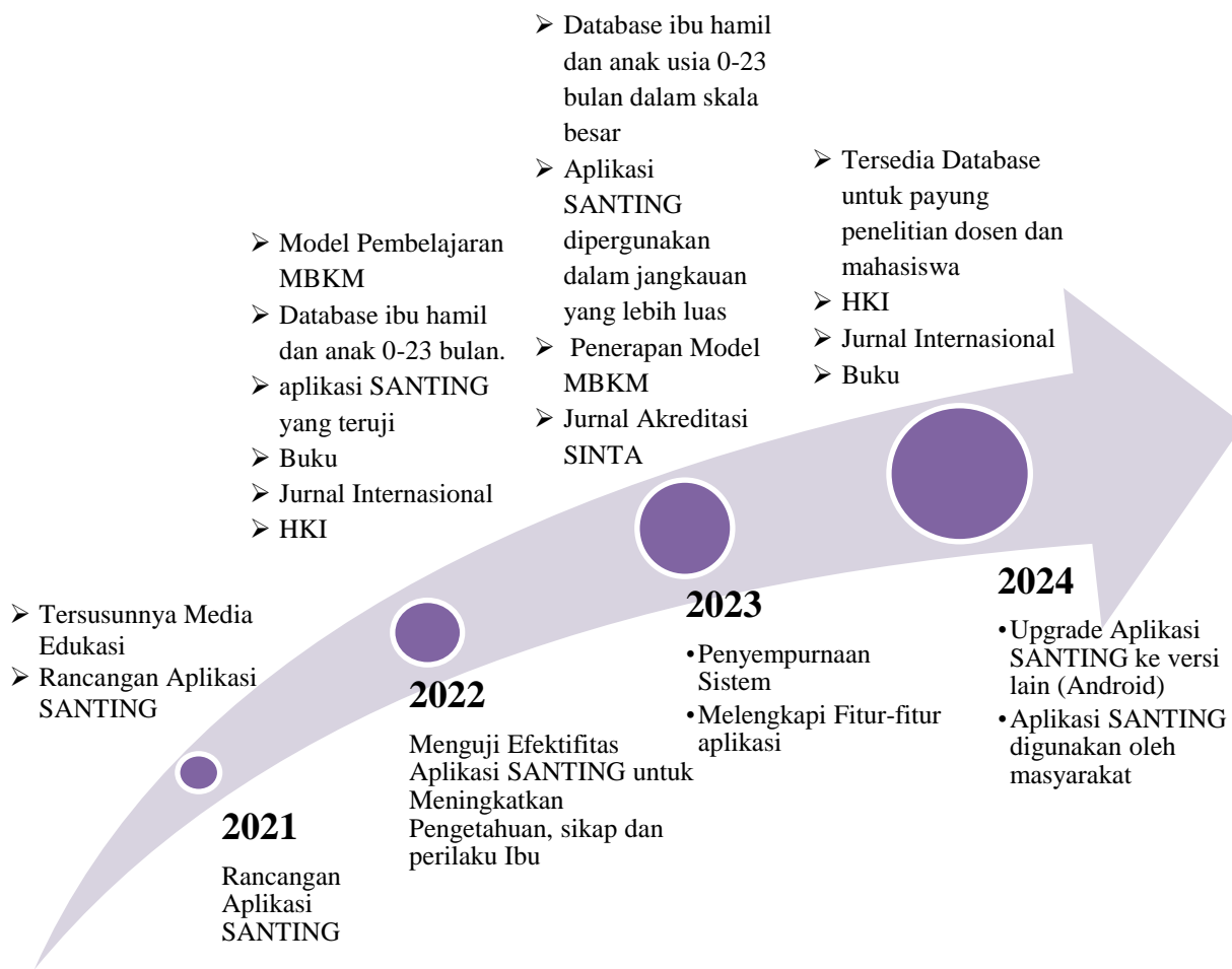
Gambar 1. Roadmap Penelitian
